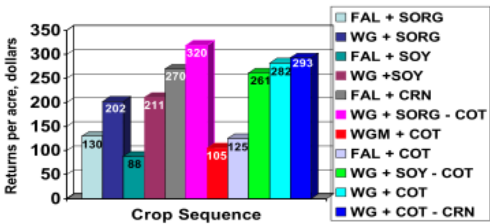
Figure 1. Annual net returns for cropping sequences in a BMP study – 2001-2006. (FAL, winter fallow; CRN, corn; WG, wheat grain; WGM, wheat green manure; SORG, grain sorghum; SOY, soybean; COT, cotton)
